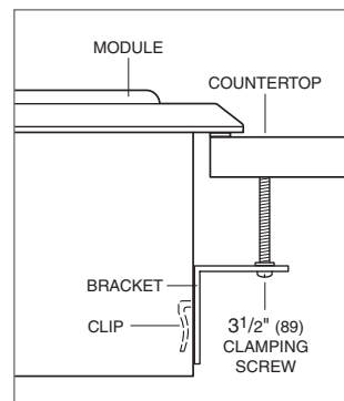
Installation brackets.
